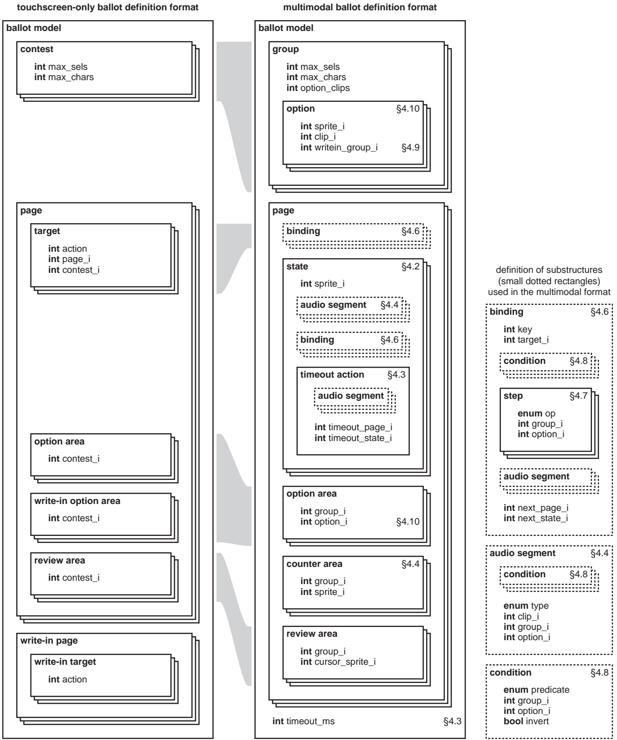
Figure 1: Side-by-side comparison of the old (touchscreen-only) and new (multimodal) ballot definition formats. Stacked rectangles represent arrays. The data structures shown in dotted rectangles are expanded on the right. Fields whose names end with _i contain array indices; in particular, sprite_i and clip_i point into arrays of images and audio clips in the video and audio sections of the ballot definition, which are not shown here. Most of the changes and additions in the new format are described in Section 4, and the relevant subsections are marked on the figure.
